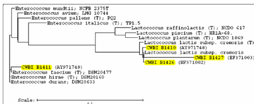
Figure 3. Dendrogramme based on similarities of 16S rDNA sequences of the bac+ isolates with those of type strains from GenBank database. GenBank accession numbers of the new bacteriocin-producing isolates are indicated in the brackets.
