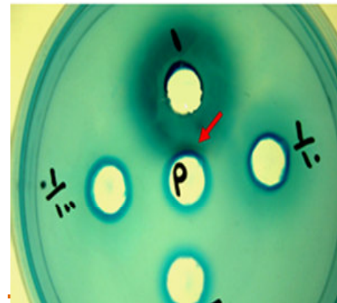
Figure 8. Immuno diffusion analysis by 1, 1:10 and 1:100 diluted DT anti toxin serum, p: Lysate of BL21 containing recombinant DT, collected 3 h after induction s: negative serum.
