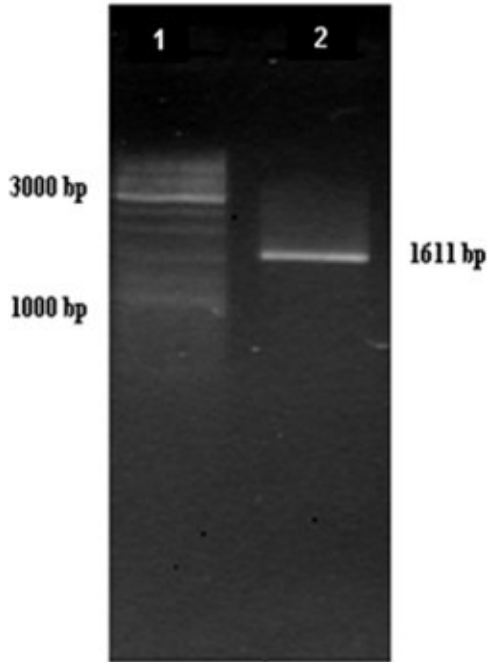
Figure 5. Electrophoresis of PCR on 1.5% agarose gel. Line 1: 100 bp DNA ladder marker. Line 2: Confirming sub cloning dt gene in pETDuet-1, expression vector (using specific primer for dt gene).
