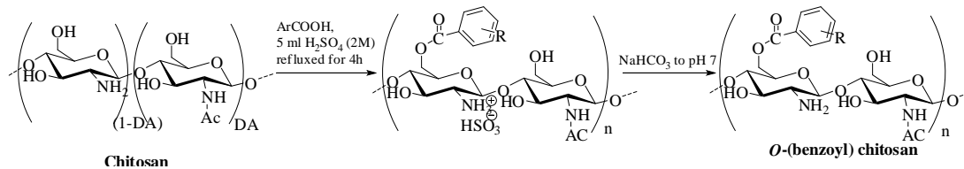
Figure 1. Synthetic route to O-(benzoyl) chitosan derivatives. DA is the degree of acetylation and Ac is the acetyl group.
