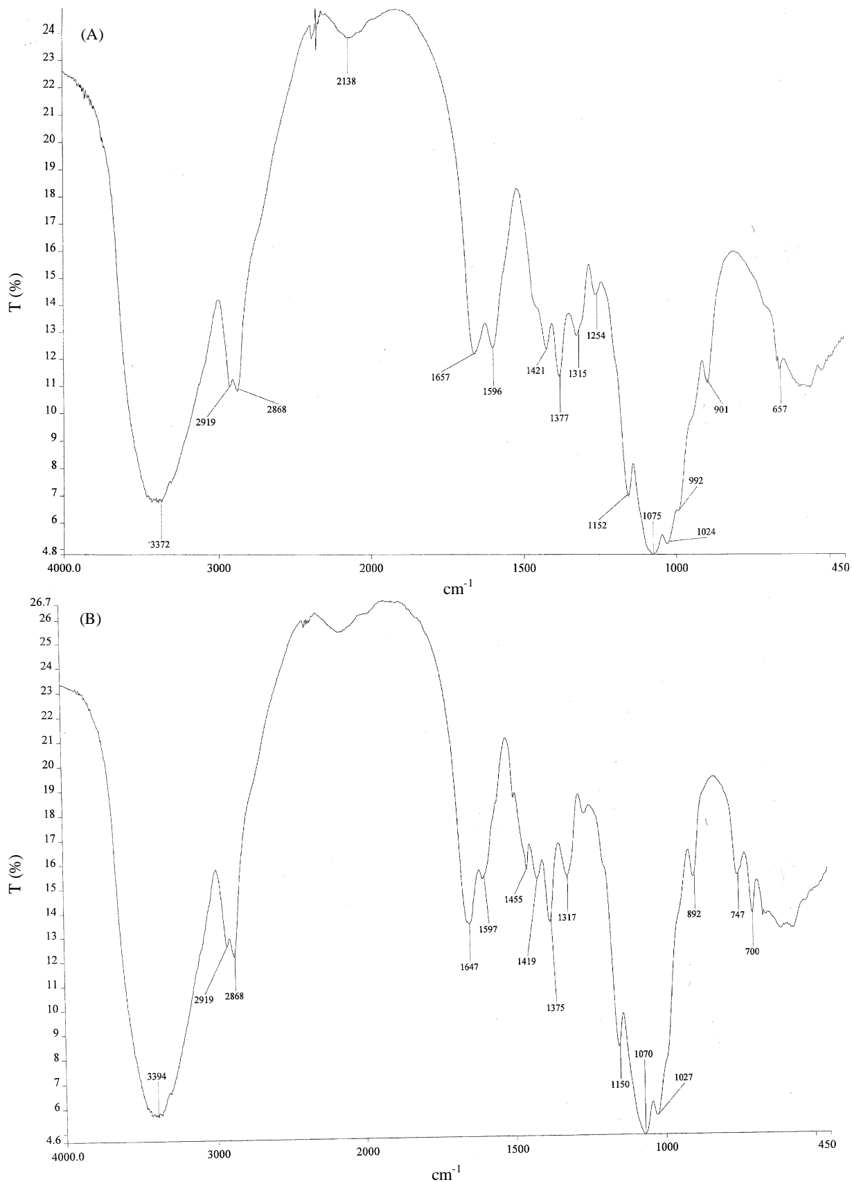
Figure 3. The FTIR spectra of chitosan (A) and O-(benzoyl) chitosan derivative (compound 1, B).
