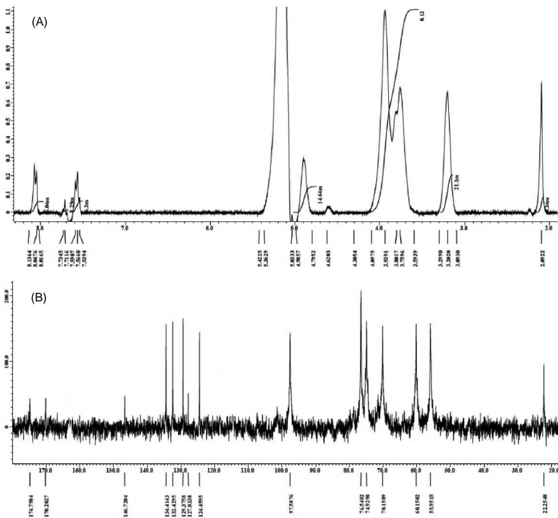
Figure 2. 1 H- and 13 C-NMR spectra of O-(benzoyl) chitosan (A and B, respectively) in 1% CD 3 COOD/D 2 O at 25°C.
