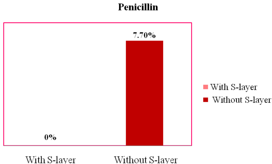
Diagram 2. Sensitive pattern into penicillin in B. cereus strains producer and non producer S-layer.
