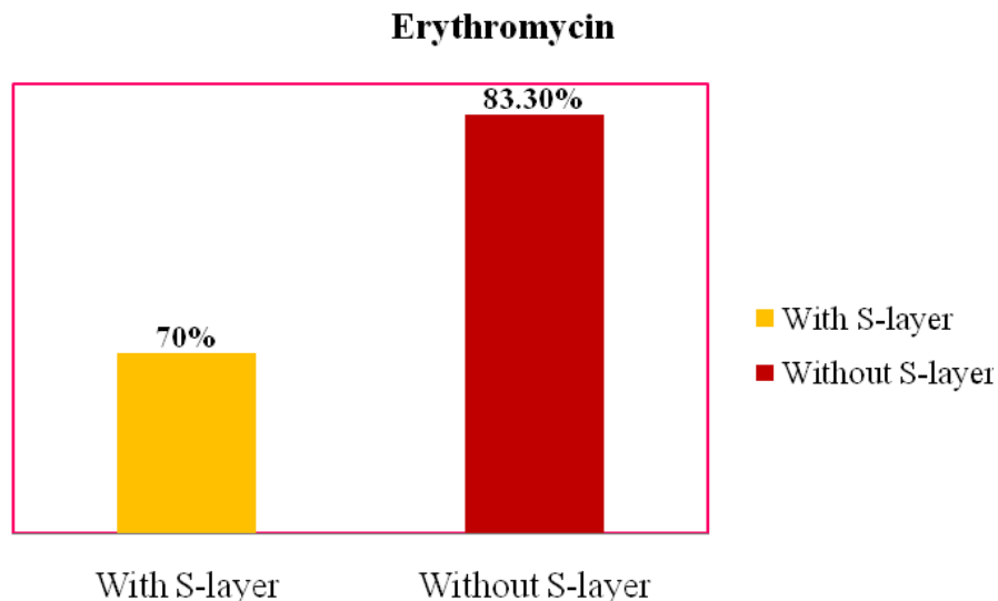
Diagram 3. Sensitive pattern into erythromycin in B. cereus strains producer and non producer S-layer.
