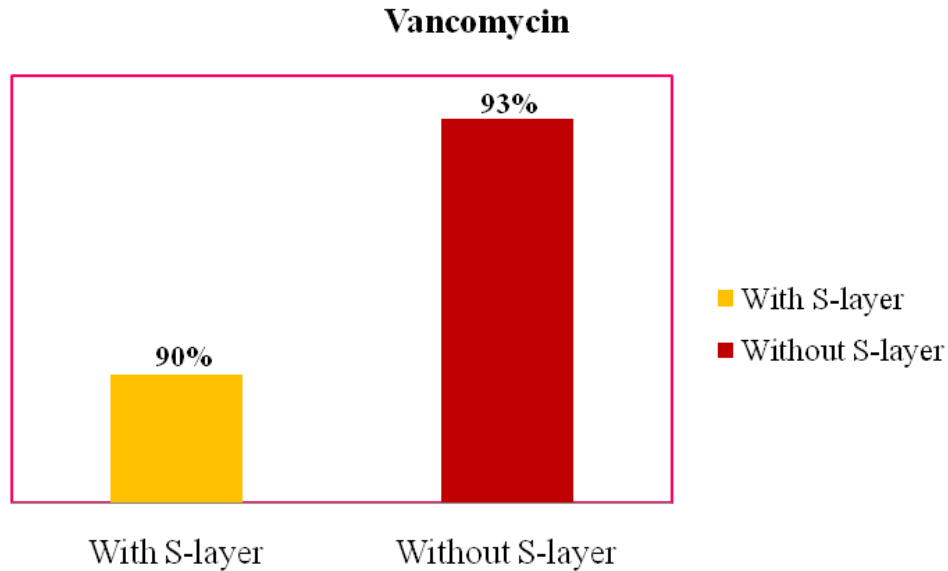
Diagram 4. Sensitive pattern into Vancomycin in B. cereus strains producer and non producer S-layer.
