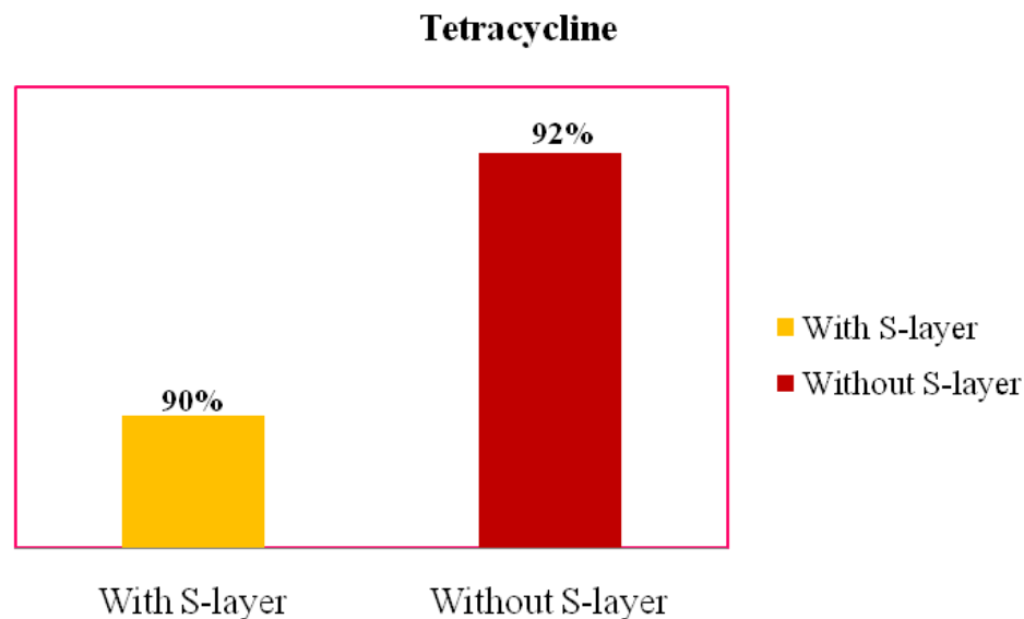
Diagram 5. Sensitive pattern into Tetracycline in B. cereus strains producer and non producer S-layer.
