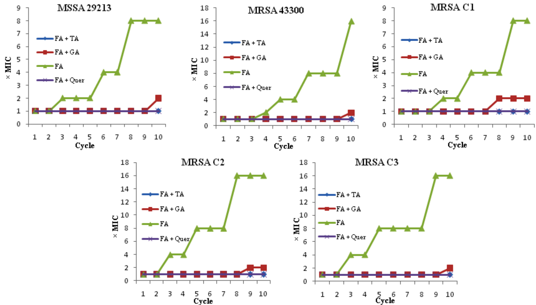
Figure 3. Selection of fusidic acid resistant S. aureus after serial exposure to fusidic alone or in combination with 0.25 × MIC of tannic acid, gallic acid ethyl ester and quercetin.
