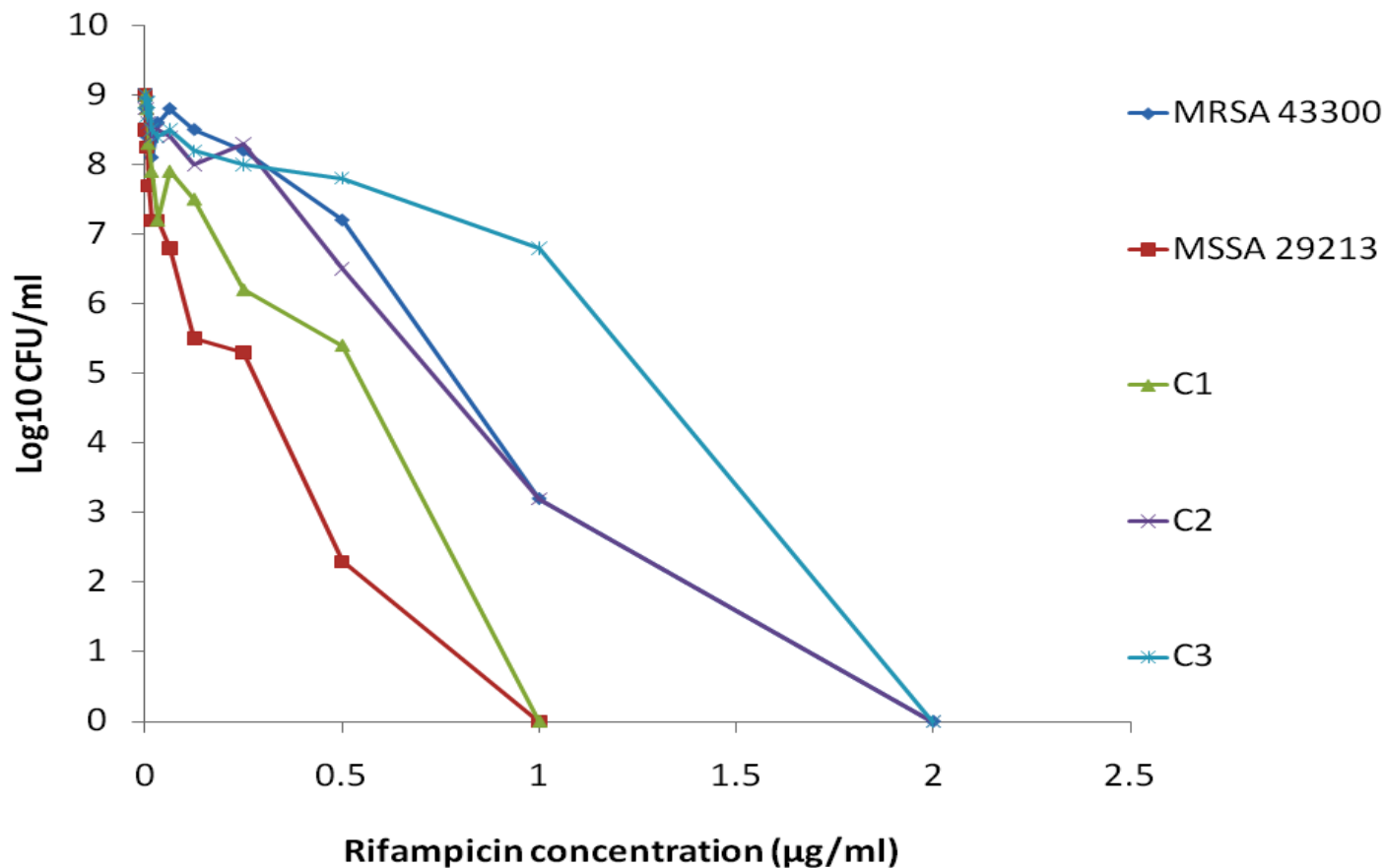
Figure 2. Population analysis profile (PAP) for rifampicin against S. aureus strains (MRSA 43300, MSSA 29213 and 3 MRSA clinical strains: C1, C2 and C3).
