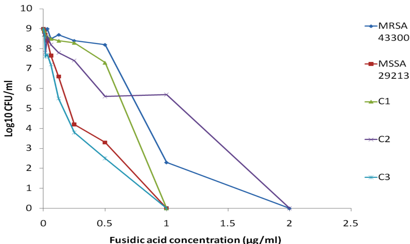
Figure 1. Population analysis profile (PAP) for fusidic acid against 5 S. aureus strains (MRSA 43300, MSSA 29213 and 3 MRSA clinical strains: C1, C2 and C3).
