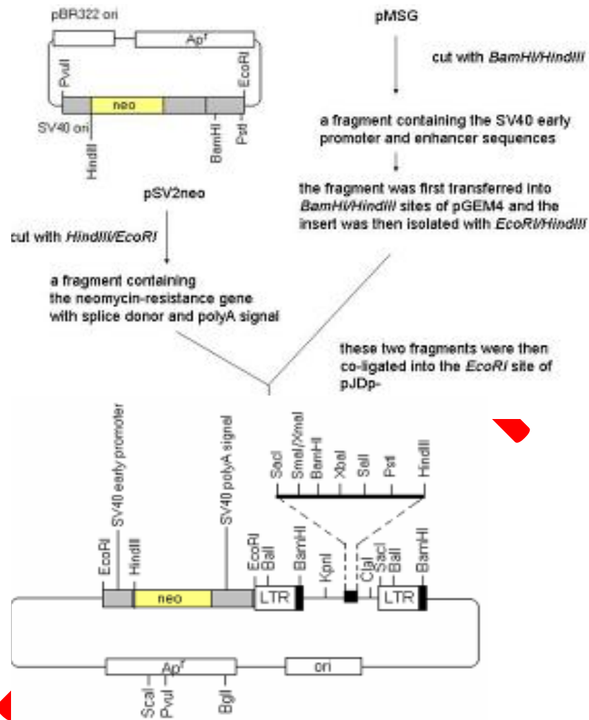
Figure 3. Vector construction and deduced restriction map of pSN.
