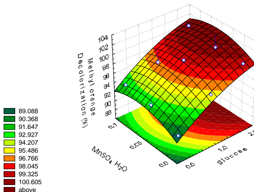
Figure 4. The interaction of glucose with \text{MnSO}_4\cdot\text{H}_2\text{O} .
