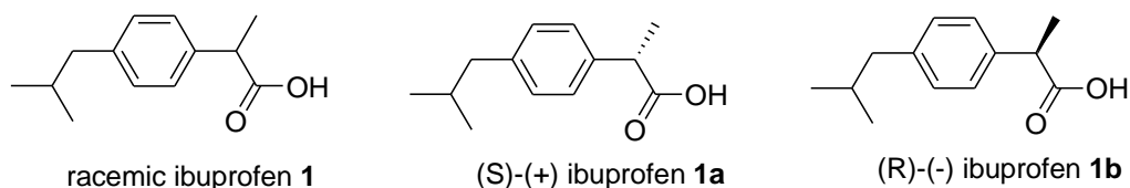
Figure 1. Racemic ibuprofen and its enantiomers.
