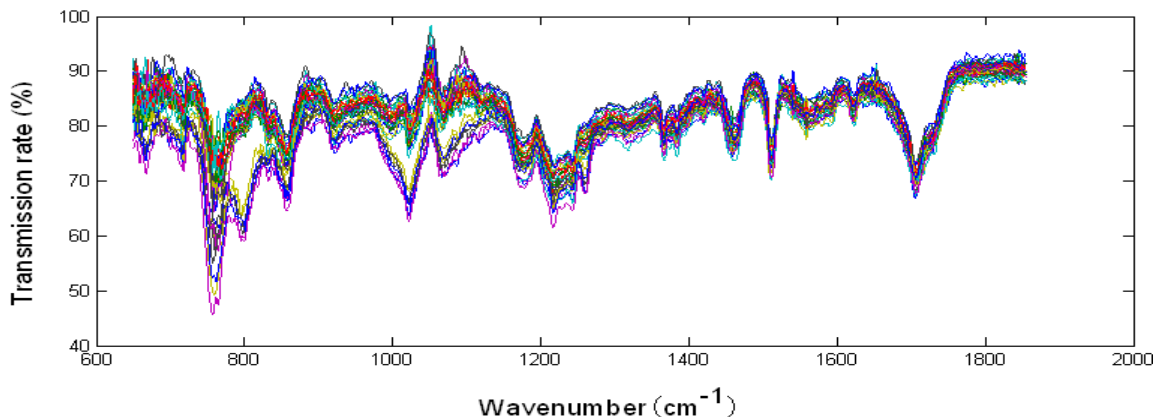
Figure 2. Original transmission spectra of different ibuprofen enantiomers.
