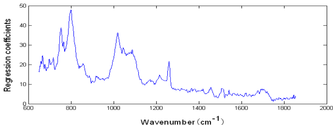
Figure 3. PLS model regression coefficients.
