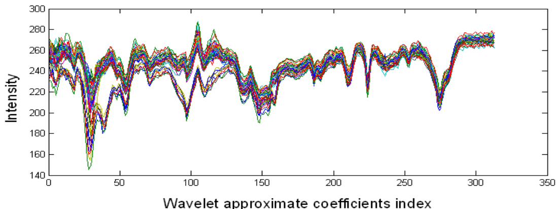
Figure 4. Wavelet approximate coefficients of ibuprofen spectral using Haar wavelet function and decomposition level 3.
