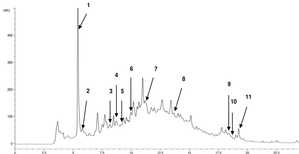
Figure 1. RP-HPLC Chromatographic profiles of phenolic acids and flavonoids in diluted acetone extract of S. persica stems monitored at 280 nm. The peak numbers correspond to: 1, caffeic acid; 2, gallic acid; 3, 3,4 dihydroxyphenylacetic acid; 4, chlorogenic acid; 5, catechine hydrate; 6, resorcinol; 7, rutine trihydrate; 8, p -coumaric acid; 9, quercitine dehydrate; 10, naphtho-resorcinol; 11, trans-cinnamic acid.
