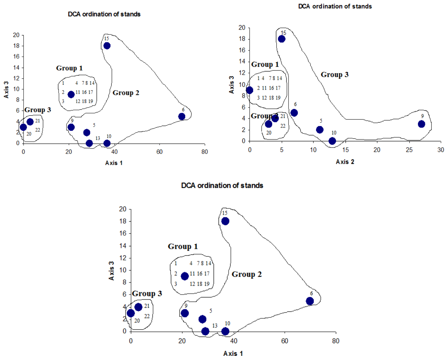
Figure 2. DCA ordination (axes 1, 2 and 3) of the 22 stands surveyed. The groups derived from Ward's cluster analysis are superimposed on the ordination space.
