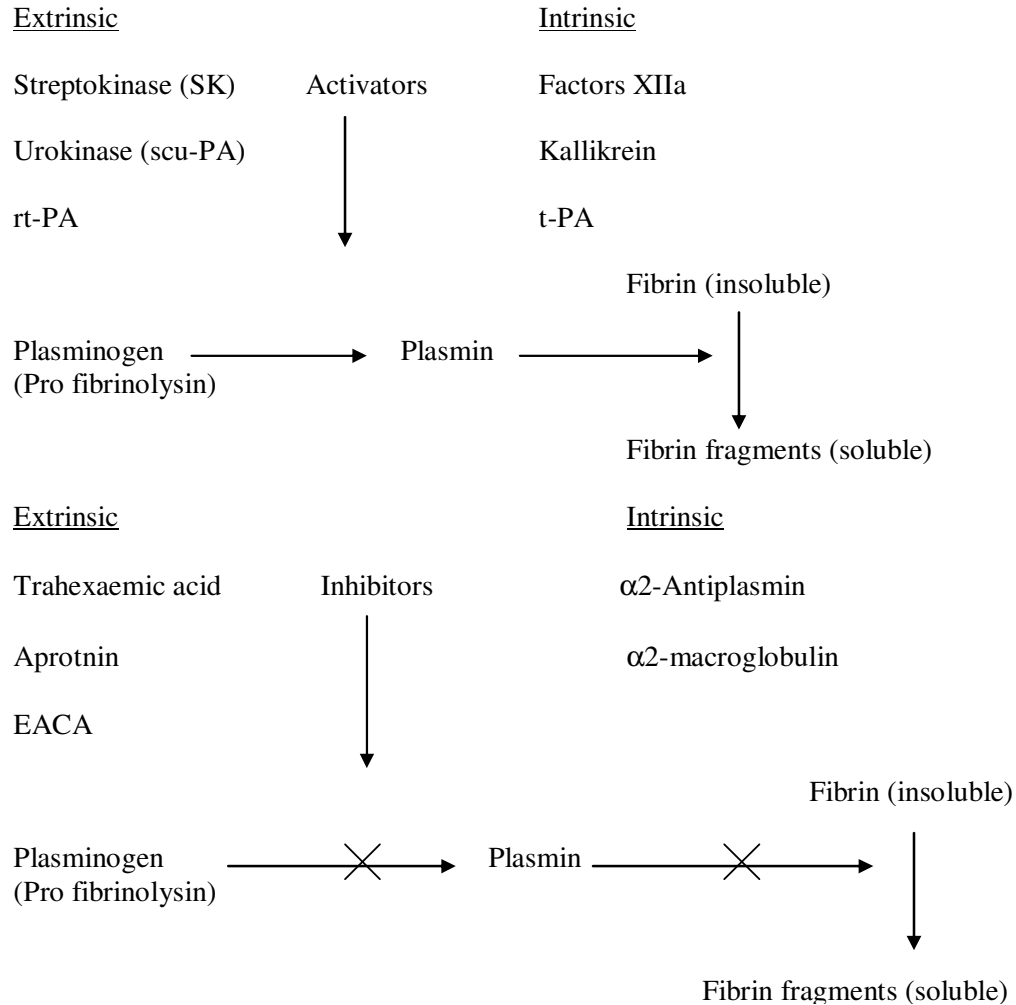
Figure 1. Relationship of components of the fibrinolytic system with activators.
