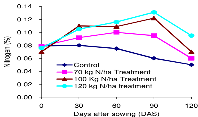
Figure 6. Nitrogen status in the soil during growing period of maize.
