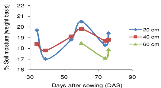
Figure 2. Soil moisture status at I 1 (IW/CPE = 0.2).
