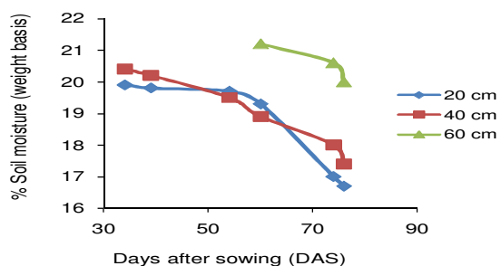
Figure 1. Soil moisture status at I 0 (IW/CPE = 0.0).
