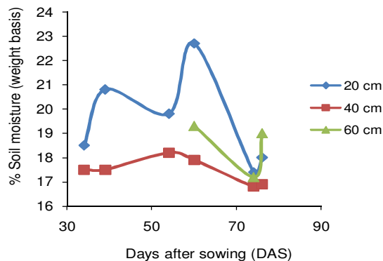
Figure 4. Soil moisture status at I 3 (IW/CPE = 0.8).
