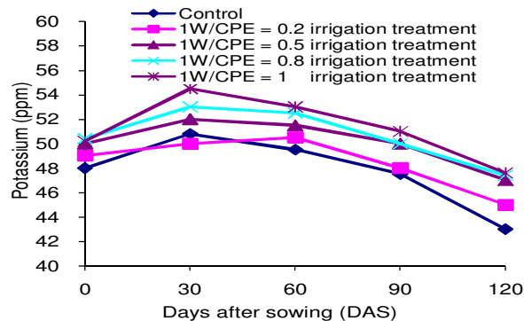
Figure 7. Potassium status in the soil during growing period of maize
