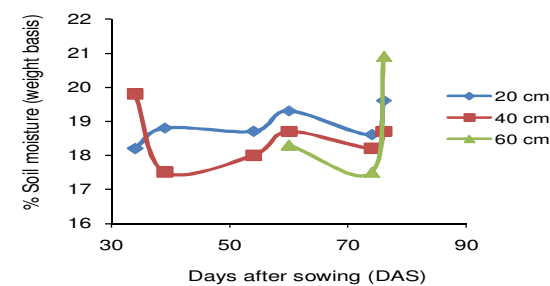
Figure 3. Soil moisture status at I 2 (IW/CPE = 0.5).
