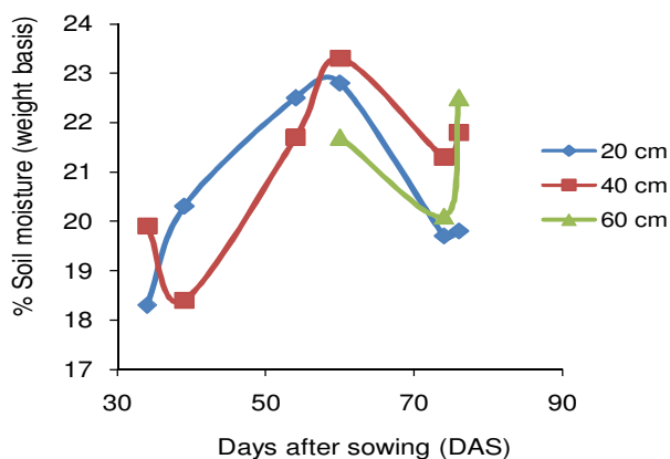
Figure 5. Soil moisture status at I 4 (IW/CPE = 1.0).
