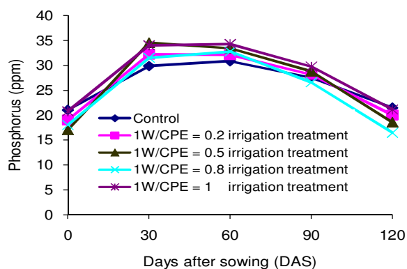
Figure 8. Phosphorus status in the soil during growing period of maize
