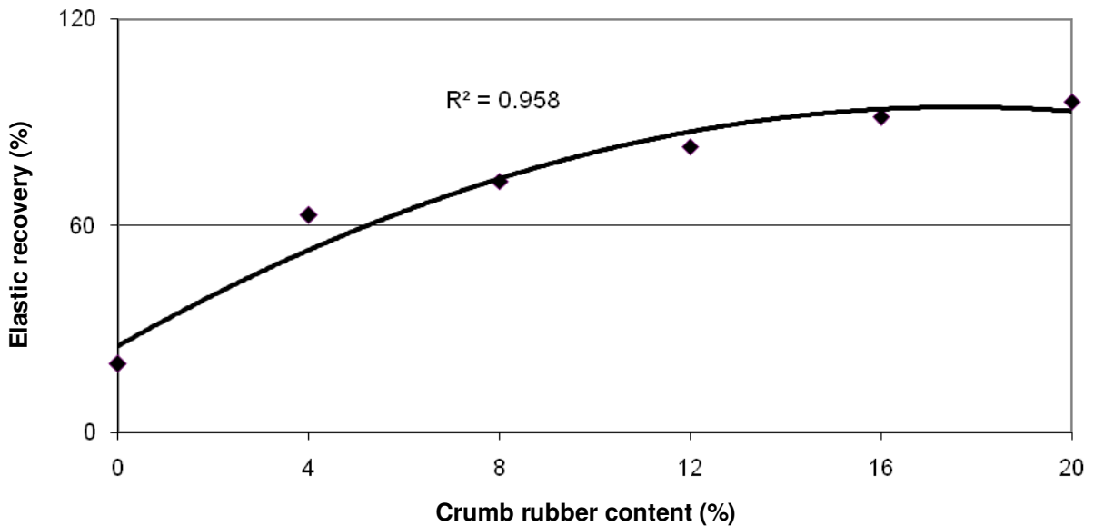
Figure 2. Elastic recovery test results for different crumb rubber content.
