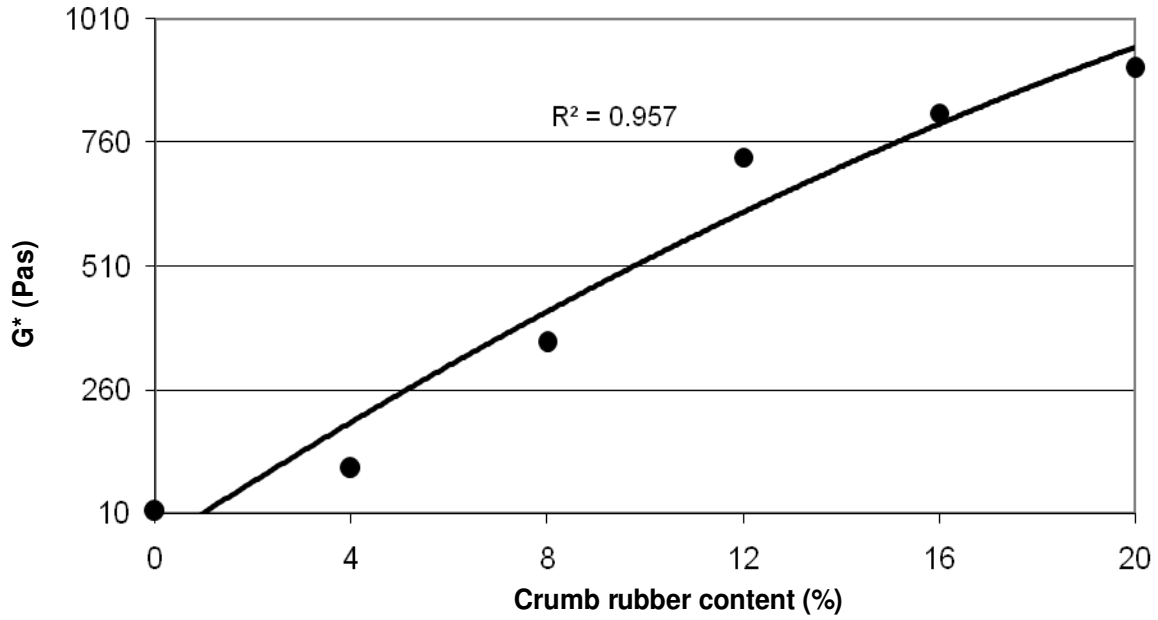
Figure 6. Storage modulus test results for different crumb rubber content.
