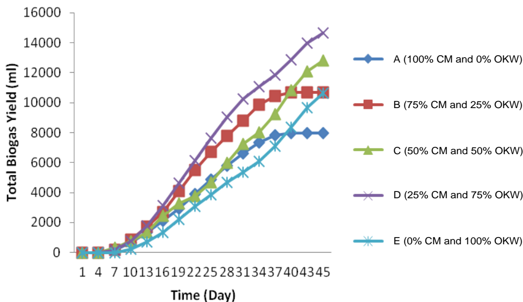
Figure 2. Mean cumulative biogas yield of all samples within 45 days.
