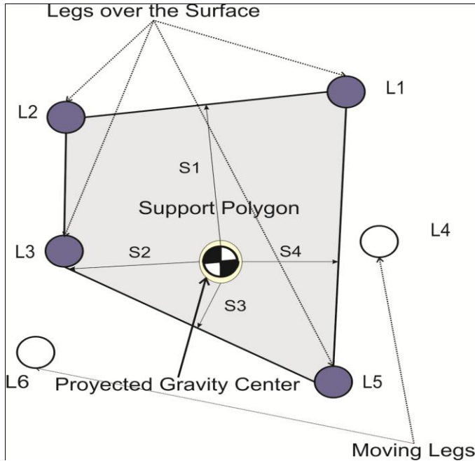
Figure 3. Diagram of six legged robot and the projection of gravity center.
