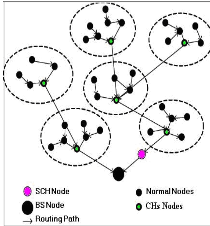
Figure 3. Hierarchical cluster formation module.
