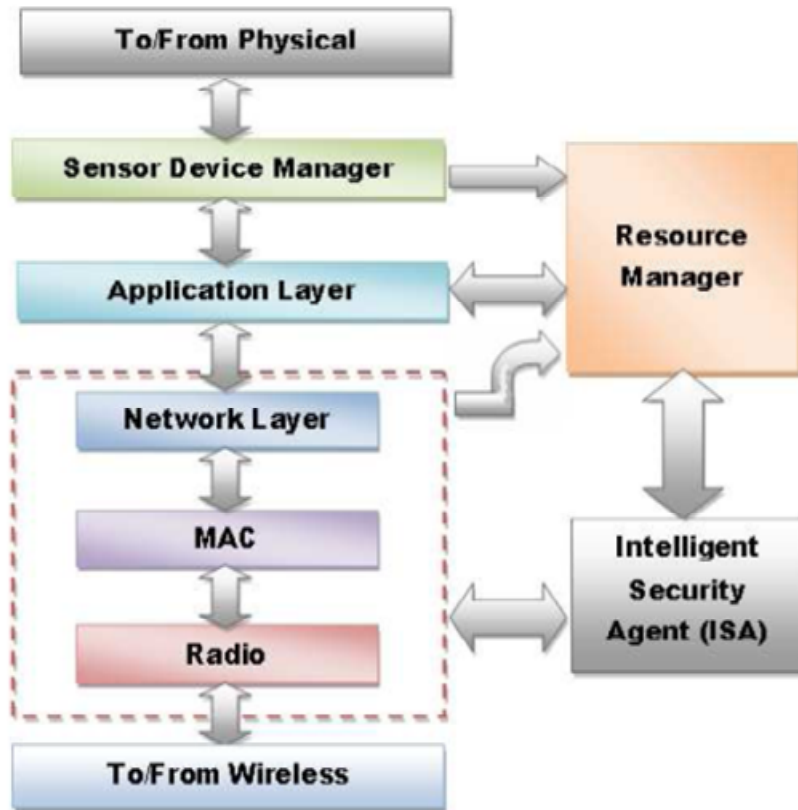
Figure 1. Coupling of ISA with protocol stack (Kalpana and Ghose, 2011).
