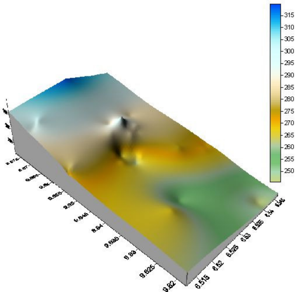
Figure 7. Digital terrain model (dtm) of the study area using surfer 8.0 software (Amadi, 2007).
