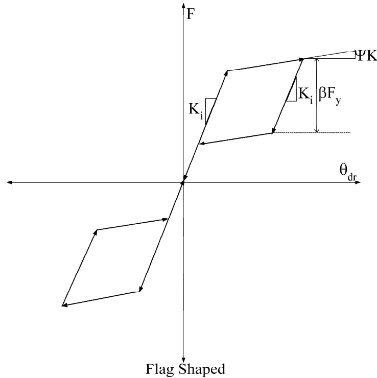
Figure 6. Flag-shaped model
