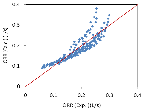
Figure 1. Variation of calculated, Equation 1, versus measured, Kassab et al. (2007), oil recovery rate, ORR, ( V_c = 0 , and H_w = 0 ).
