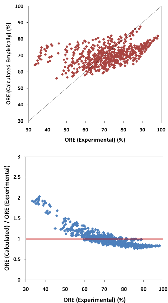
Figure 8. Comparison between the calculated, Equation 8, and the measured, Kassab et al. (2006), oil recovery efficiency, ORE for the general case: V , T , \theta , V_c and H_w are all varied.
