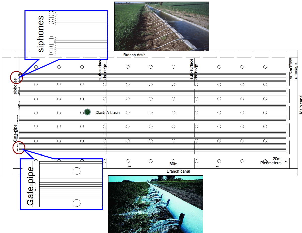
Figure 1. Experimental layout.
