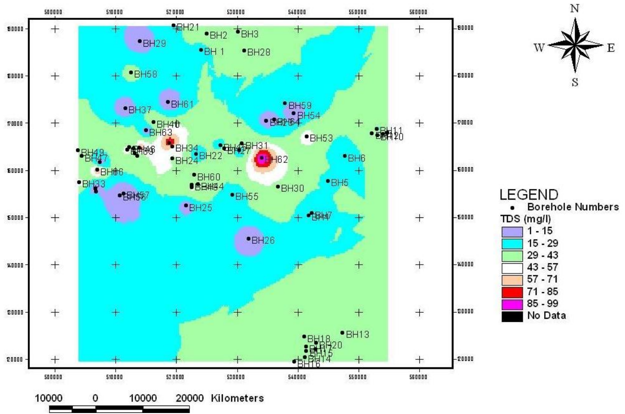
Figure 5. Spatial variation of total dissolved solid in the study area.
