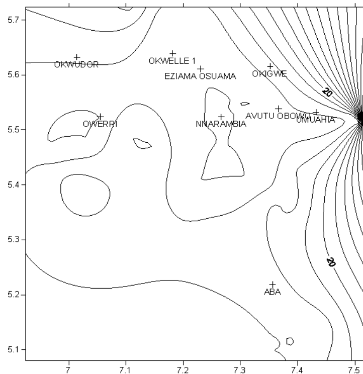
Figure 6. Contour map of turbidity in the the study area (C. I. = 5NTU).
