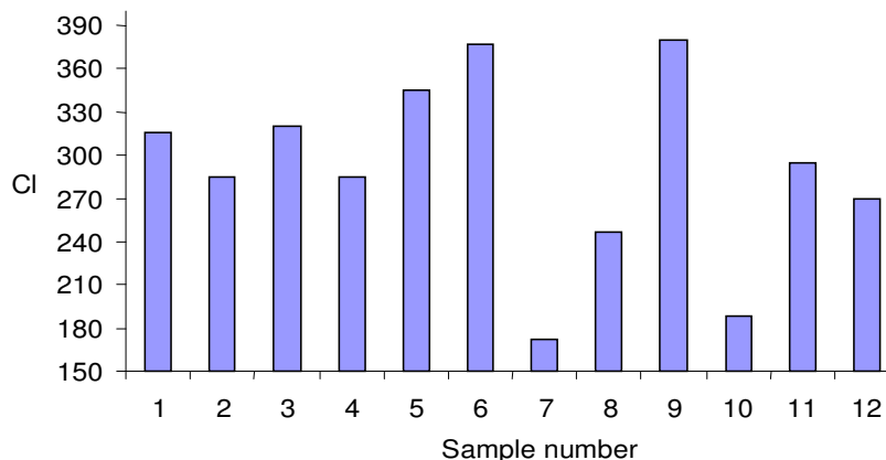
Figure 6. Cl concentration (mg/L) in ground water.
