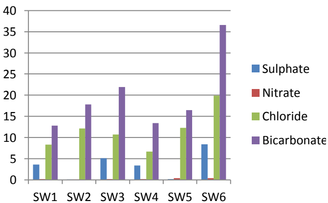
Figure 3. Major anions in the analyzed samples expressed as a bar chart.
