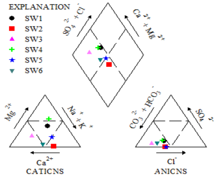
Figure 5. Piper trilinear diagram of the studied water samples.
