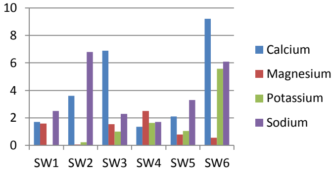
Figure 2. Major cations in the analyzed samples expressed as a bar chart.
