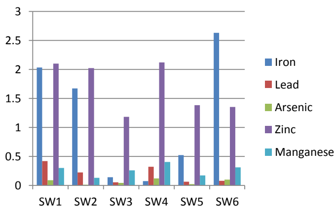
Figure 4. Trace elements concentration in the analyzed samples expressed as a bar chart.
