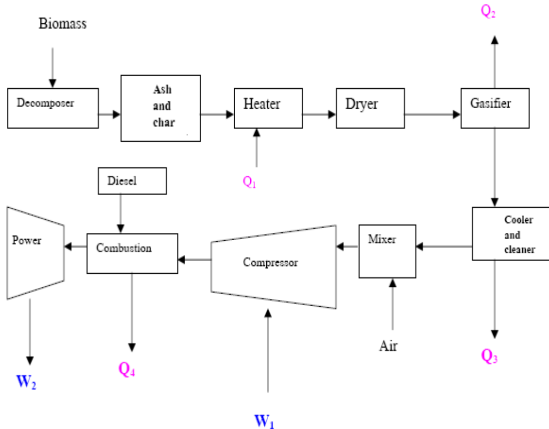
Figure 7. Advanced biomass power with diesel engine (Omer, 2006).
