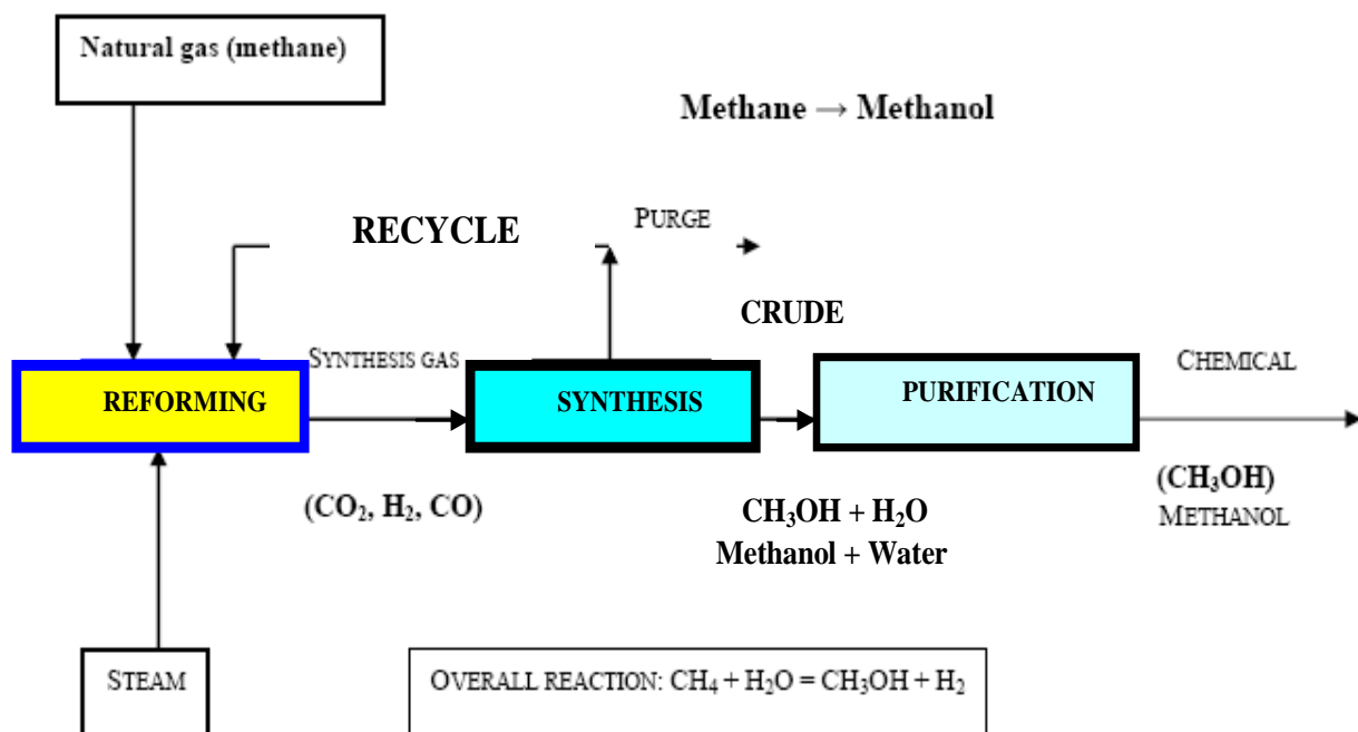
Figure 2. Schematic diagram shows methanol production (Omer, 2006).
