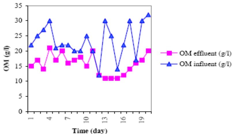
Figure 5. Organic matters before and after treatment in digester (Omer, 2006).
