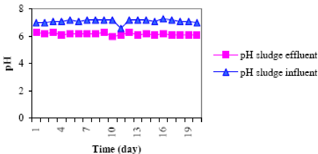
Figure 6. pH sludge before and after treatment in the digester (Omer, 2006).
