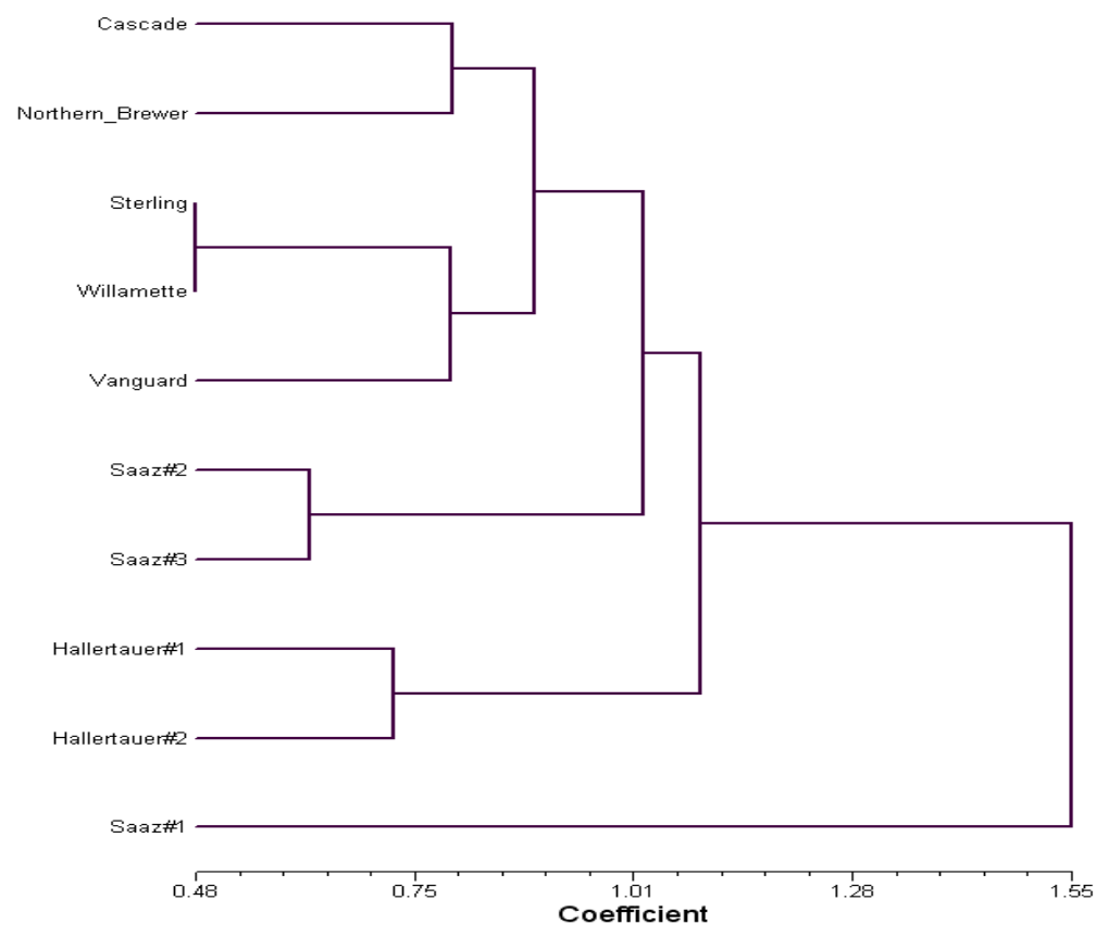
Figure 1. Dendrogram obtained by cluster analysis of the percentage composition of essential oils from finishing hops samples, based on correlation and using the Unweighted Pair-Group Method with Arithmetic Average (UPGMA).
