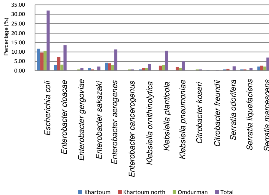
Chart 1. Percentage of Coliform organisms isolated from the vendor and market milk from Khartoum State.
