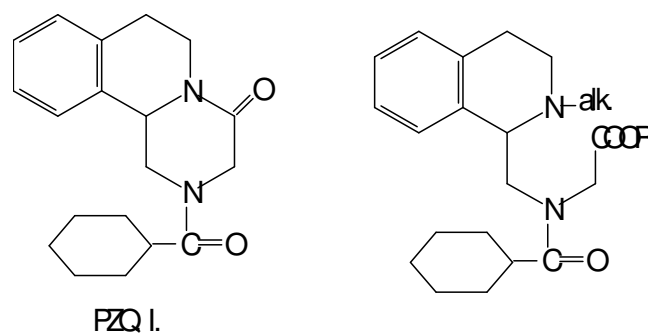
Figure 2. Chemical structure of the tested compounds.
