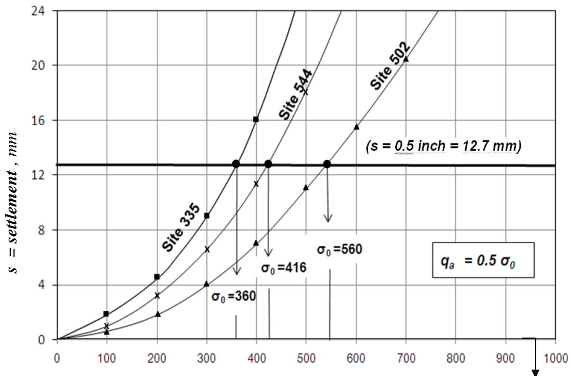
Figure 4. Load test results at Sites No: 335, 502, and 544. \sigma = pressure under the test plate, kPa; ( \sigma_0 = 2 q_a = pressure, which produces s = 12.7 mm).
