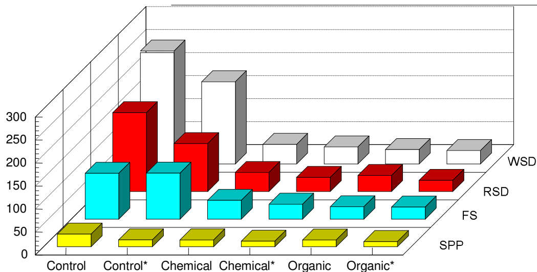
Figure 1. Changes in C/N ratio of different raw materials used during composting. *Biofortified with cellulose decomposing microorganisms; Spp = Sheath of peanut pods, FS= Flax shiver, RSD= Red sawdust, WSD= White sawdust.
