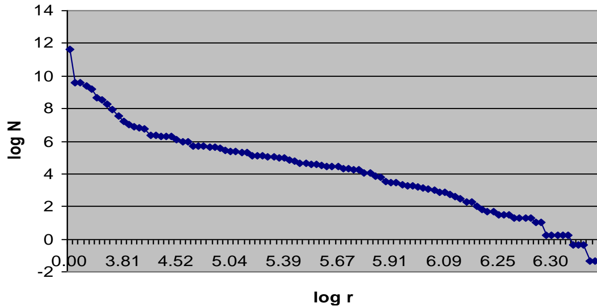
Figure 4. Diagram rank-frequency of the distribution of the woody species in the savannas.
