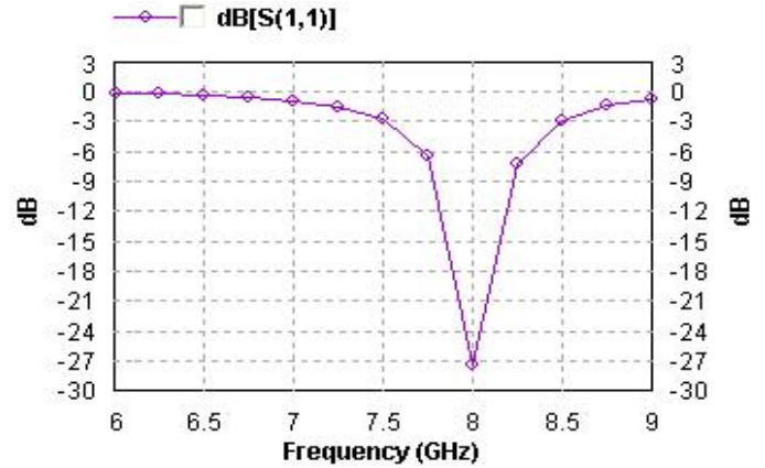
Figure 2. The return loss (S 11 ) in dB verses resonating frequency of microstrip antenna.
