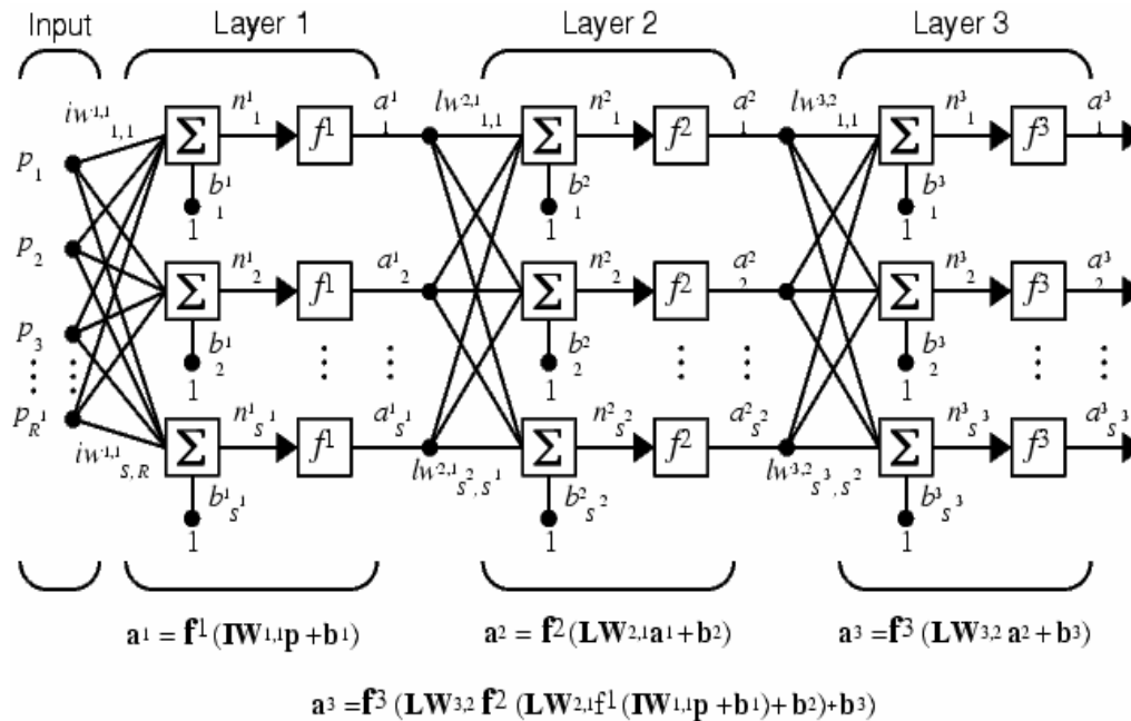
Figure 3. Three layer feed forward artificial neural network.
