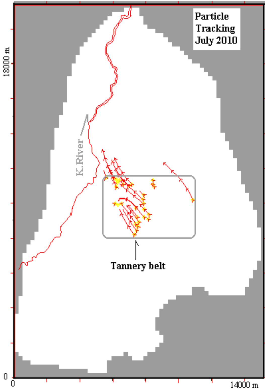
Figure 10. Streamlines migration predicted up to 2010 since 1988.
