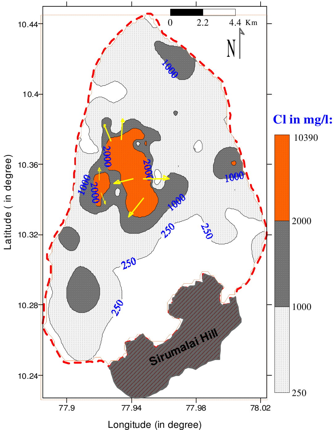
Figure 5. Cl shaded map (January 2001)
