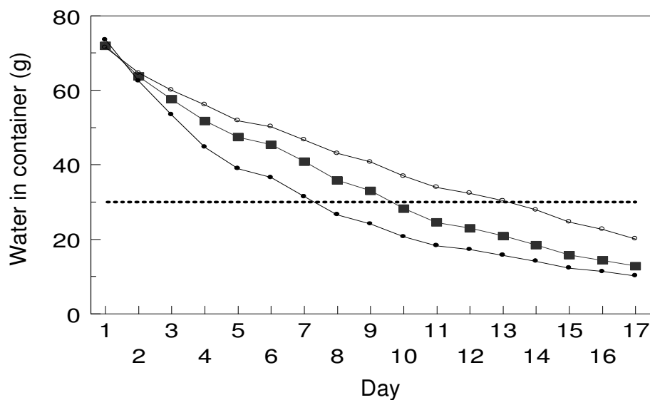
Figure 1. Effect of clipping treatment on water remaining in the media + seedling. 28-NoClip = bottom line, solid circle, 15-Clip = solid square, 5-Clip = top line, open circle
