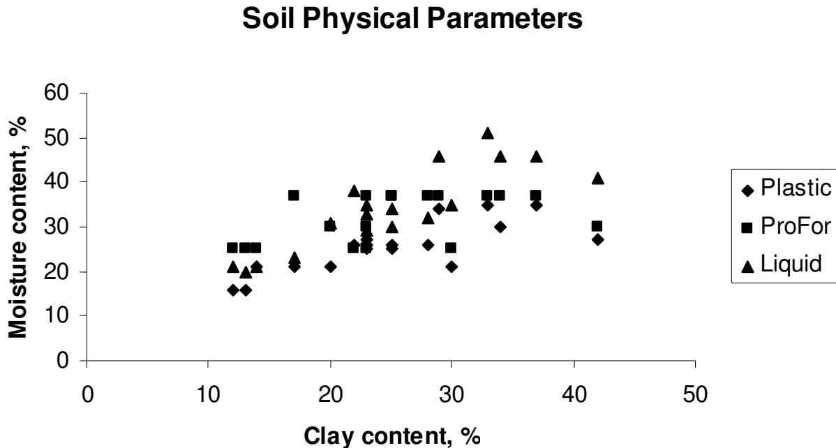
Figure 4. Relationship between the soils clay content, plastic limits, liquid limits and the predicted critical soil moisture contents.
