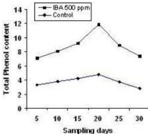
Figure 5. Total phenol content in different time period of root development from cuttings of Saroca asoca pretreated with or with out IBA (500 ppm). The phenol content was expressed as mg/gm. fresh weight. Values are means \pm SE.
