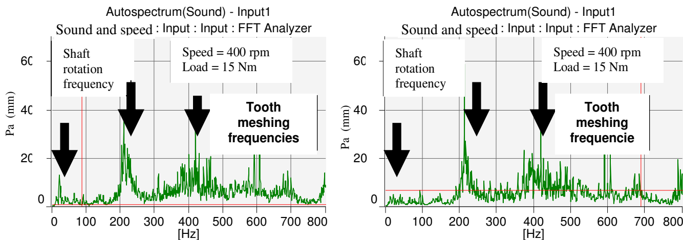
Figure 10. Locations of tooth meshing and shaft rotation frequencies: a) Healthy gear; b) Faulty gear (g4), 3.0 × 0.5 × 40 mm.
