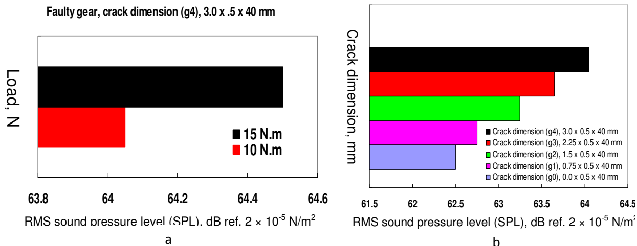
Figure 9. RMS sound pressure level: a) Influence of load; b) Influence of crack dimension.
