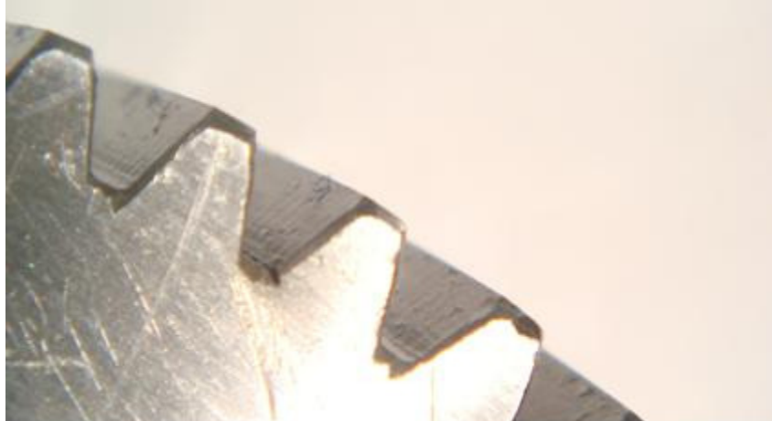
Figure 4. Gear tooth crack.
