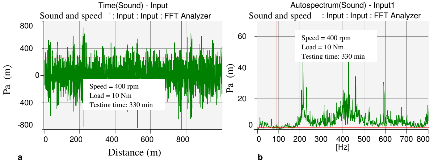
Figure 11. Sound pressure level spectra: a) Time history (g4), 3.0 × 0.5 × 40 mm; b) Frequency domain (g4), 3.0 × 0.5 × 40 mm.
