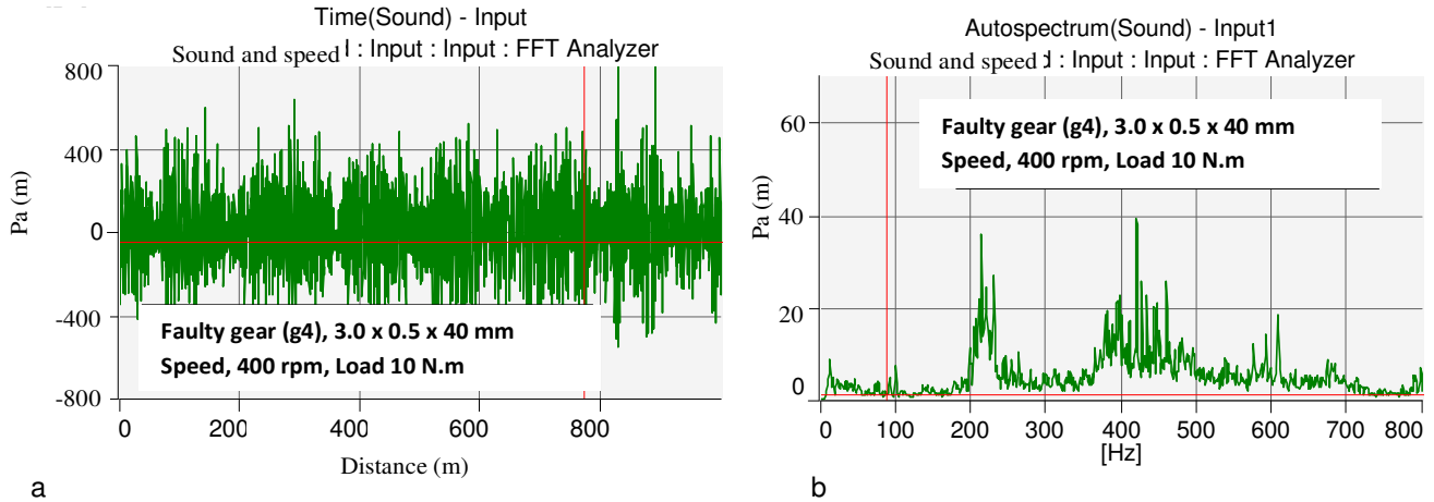
Figure 7. Sound pressure level spectra: (a) Time history of sound pressure level; b) Frequency domain of sound pressure level.
