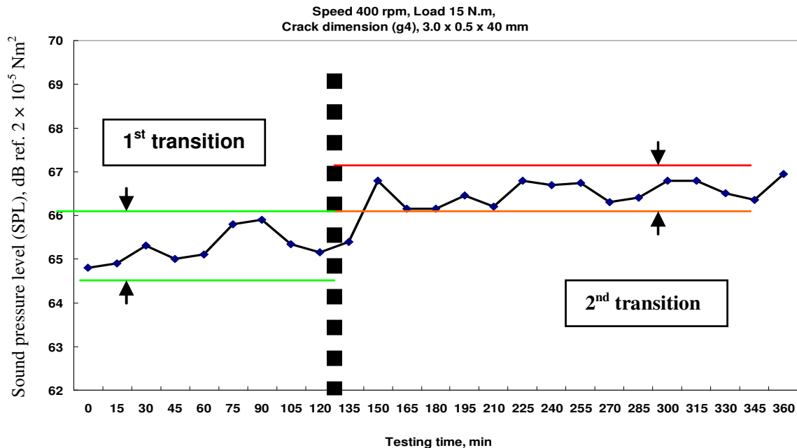
Figure 13. Relationship between RMS of SPL and testing time.
