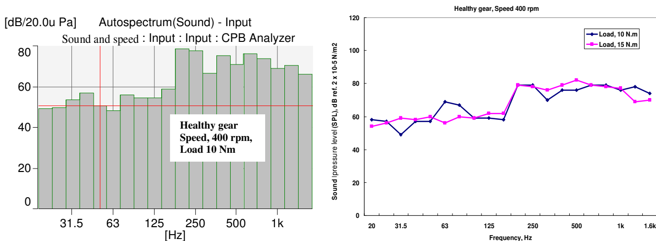
Figure 6. 1/3-Octave sound pressure level spectra. a) 1/3-octave sound pressure level. b) 1/3-octave sound pressure level.
