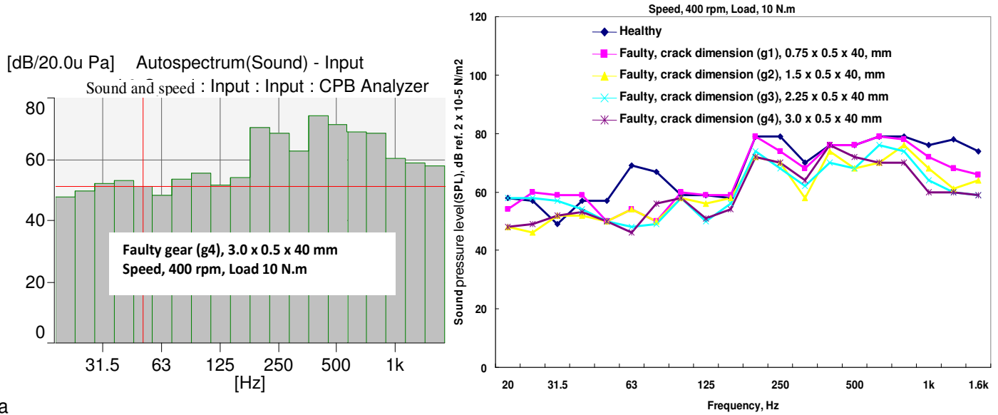
Figure 8. 1/3-Octave sound pressure level spectra: a) 1/3-octave sound pressure level; b) 1/3-octave sound pressure level.
