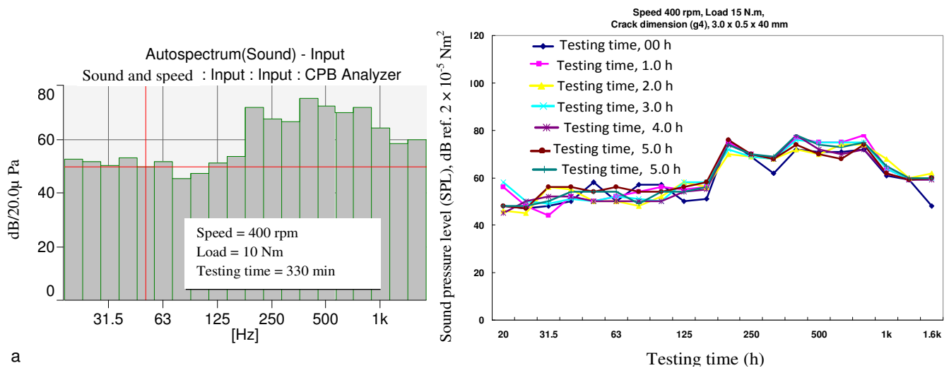
Figure 12. 1/3-Octave sound pressure level spectra. a) 1/3-octave sound pressure level. b) 1/3-octave sound pressure level.
