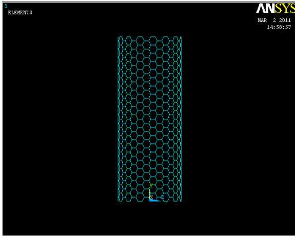
Figure 6. Meshed structure (armchair).
