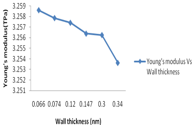
Figure 11. Shows the variation of Young's modulus with wall thickness.
