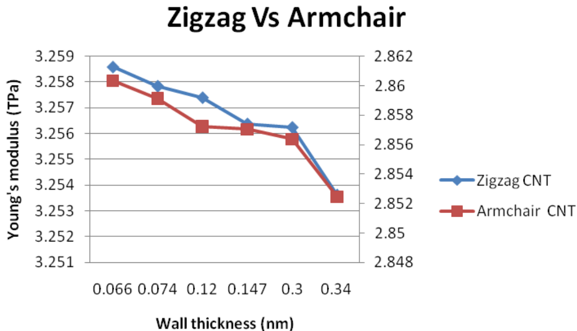
Figure 12. Zigzag Vs Armchair CNT.
