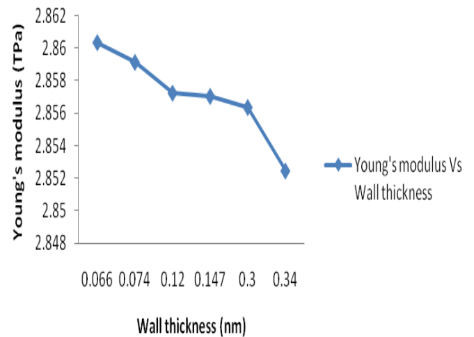
Young's modulus Vs Wall thickness (Armchair type CNT)
