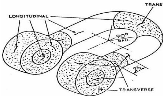
Figure 8. Shackle reprinted from IS 7587 (Part 1): 2004 [G]
