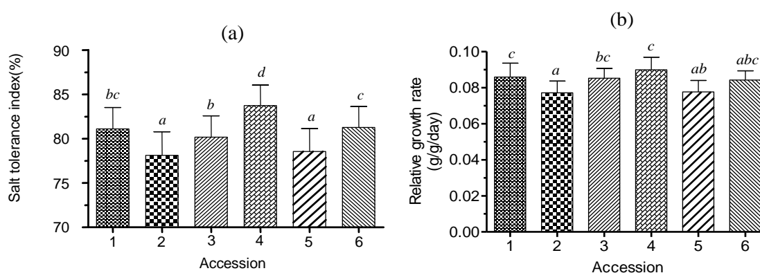
Figure 1. Salt tolerance index (a) and relative growth rate (b) of six accessions of A. paniculata under different salinity levels of NaCl (control, 4, 8, 12, and 16 dSm -1 ) and various exposure times (5, 10, 15, and 20 days). Mean values \pm standard error (SE) are from three independent replicates. Values superscripted by different letters are significantly different ( P \leq 0.01 ). The accessions were: (1) 11179, (2) 11216, (3) 11241, (4) 11249, (5) 11264, and (6) 11329.
