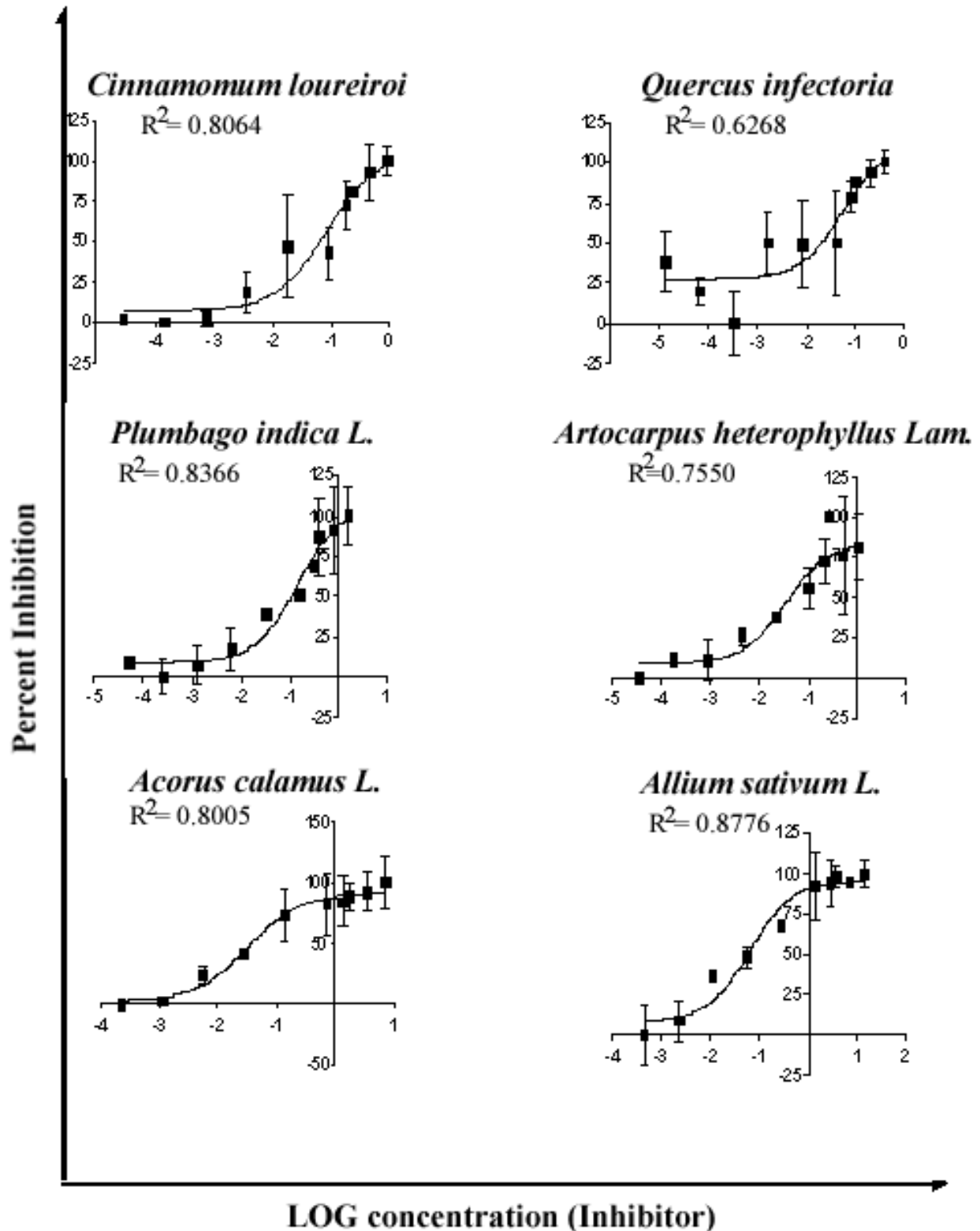
Figure 3. Nonlinear regression dose-response plot determining IC_{50} values of some plant extracts; curve and IC_{50} were automatically determined by a computer program. Values were calculated using the following equation:
