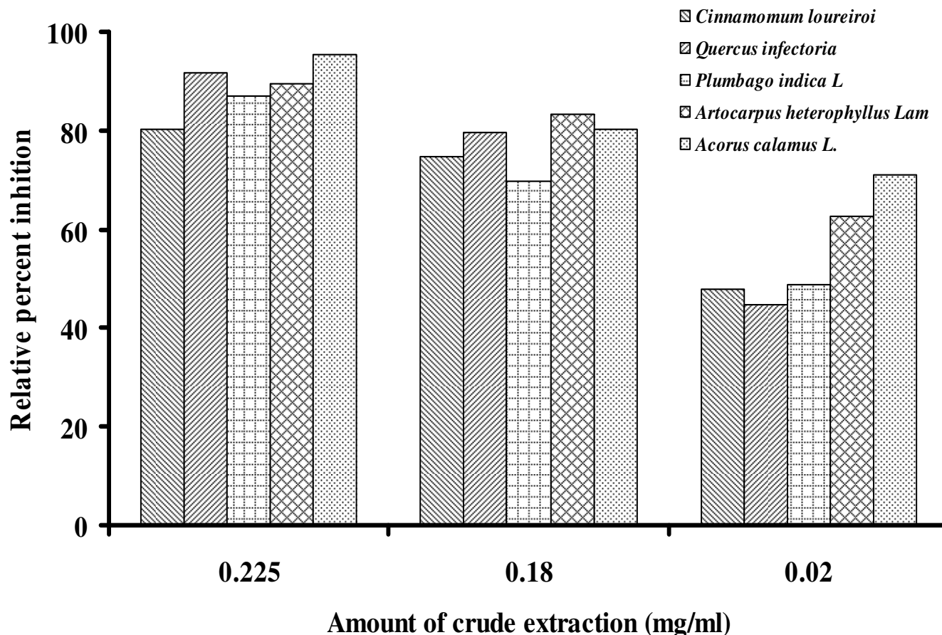
Figure 2. Increased inhibitory effect was related to concentration of crude compounds: inhibition of HIV-1 RT activity versus concentration of extracts from Acorus calamus , Artocarpus heterophyllus Lam., Quercus infectoria , Allium sativum L., Ocimum sanctum L., Cinnamomum loureiroi and Plumbago indica L.
