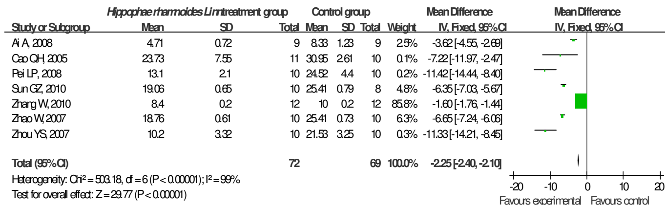
Figure 1. Forest plot comparing FBG level in the Hippophae rhamnoides Linn. treatment group compared to the model control group.
