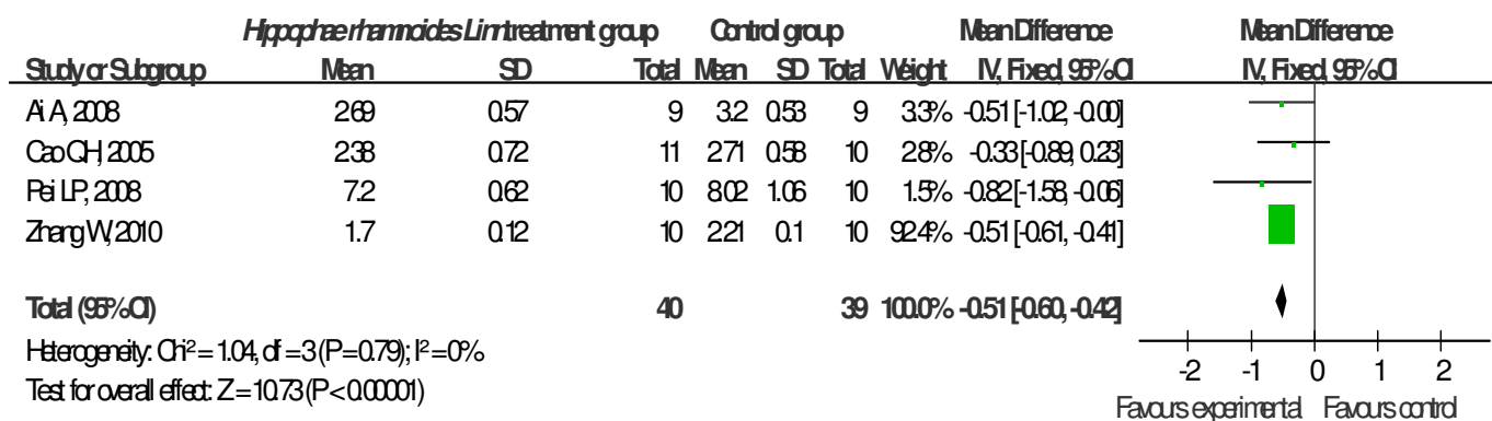
Figure 2. Forest plot comparing cholesterol level in the Hippophae rhamnoides Linn. treatment group compared to the model control group.
