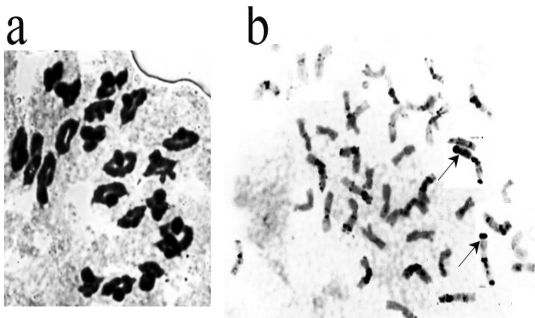
Figure 2. Cytological analysis of 6 wheat lines. (a) 21 cycle bivalents of 6 wheat lines at meiotic metaphase I (Only 96-132-1 is shown); (b) C-banding of 6 wheat lines (Only 96-132-1 is shown). Arrows show the 1BL.1RS chromosomes.
