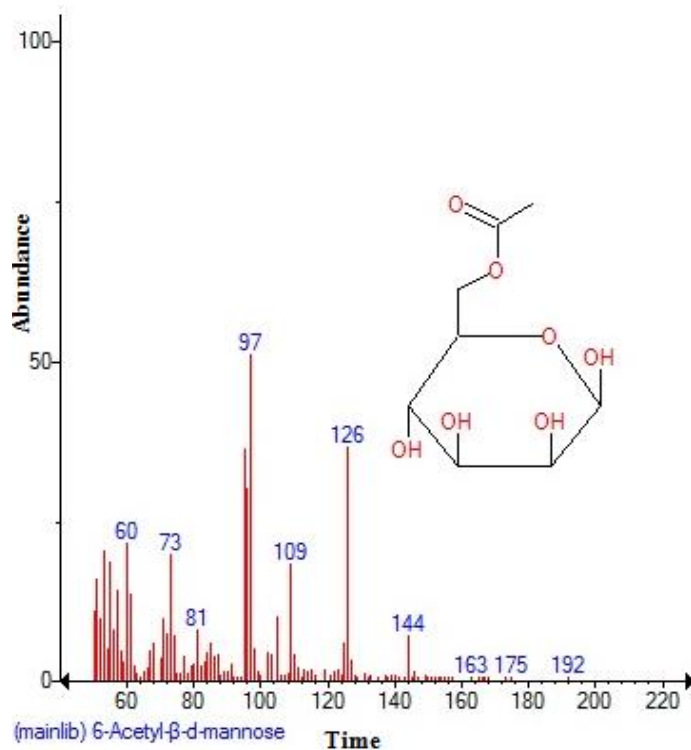
Figure 16. Structure of 6-Acetyl- \beta -D-mannose with 6.932 (RT) present in Ocimum basilicum .
