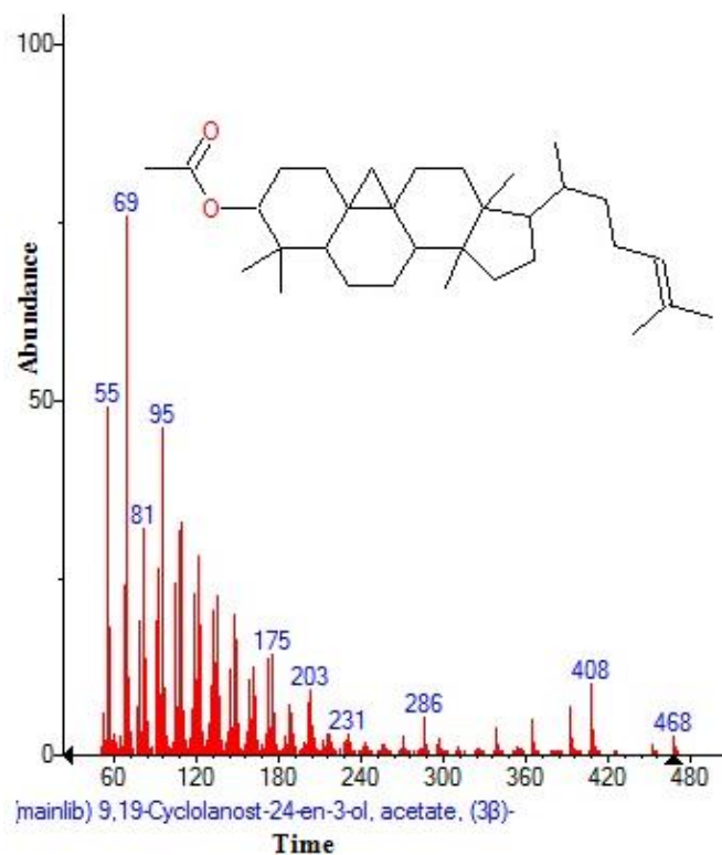
Figure 27. Structure of 9,19-Cyclolanost-24-en-3-ol, acetate, (3B) with 23.497 (RT) present in Ocimum basilicum .
