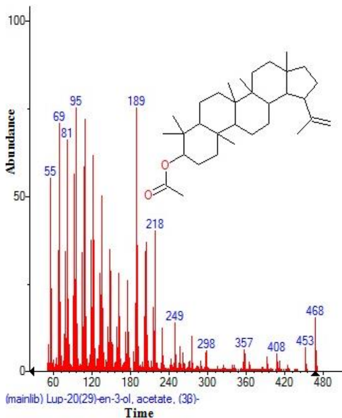
Figure 29. Structure of Lup-20(29)-en-3-ol,acetate,(3 \beta -) with 26.467 (RT) present in Ocimum basilicum .
