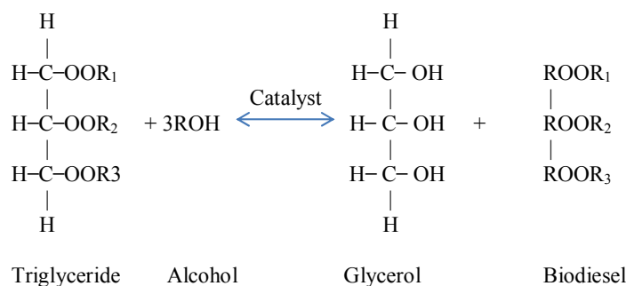
Figure 1. Transesterification of oil with methanol.
