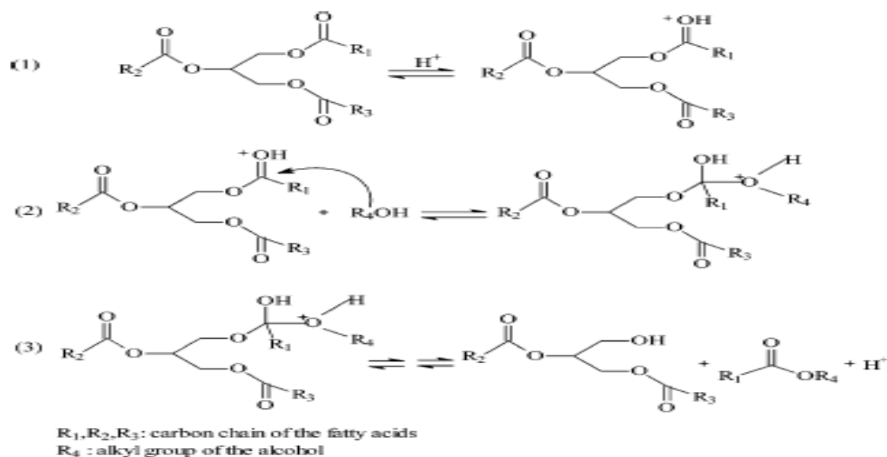
Figure 4. Mechanism of the Homogeneous acid-catalyzed reaction.
