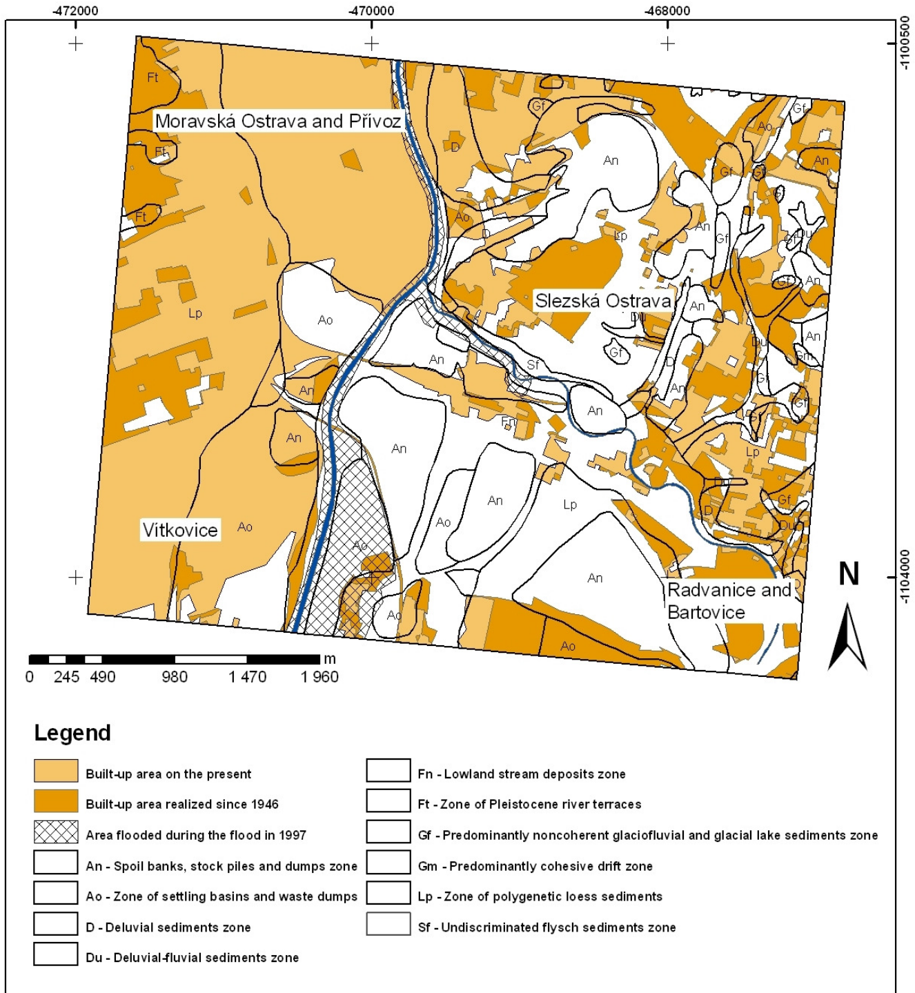
Figure 6. Map of the area flooded during the flood in 1997 with marked changes in the built-up area and engineering-geological zones.
