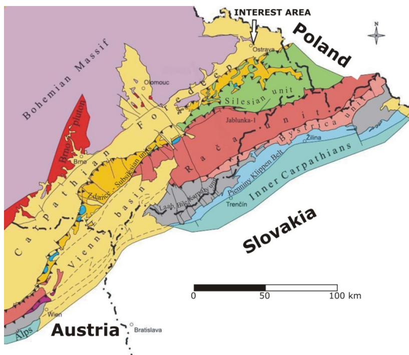
Figure 2. Schematic geological map with position of interest area.
