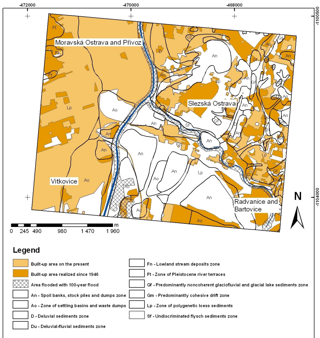
Figure 5. Map of the area flooded with 100-years flood and area flooded with 100-years flood with marked changes in the built-up area and engineering-geological zones.
