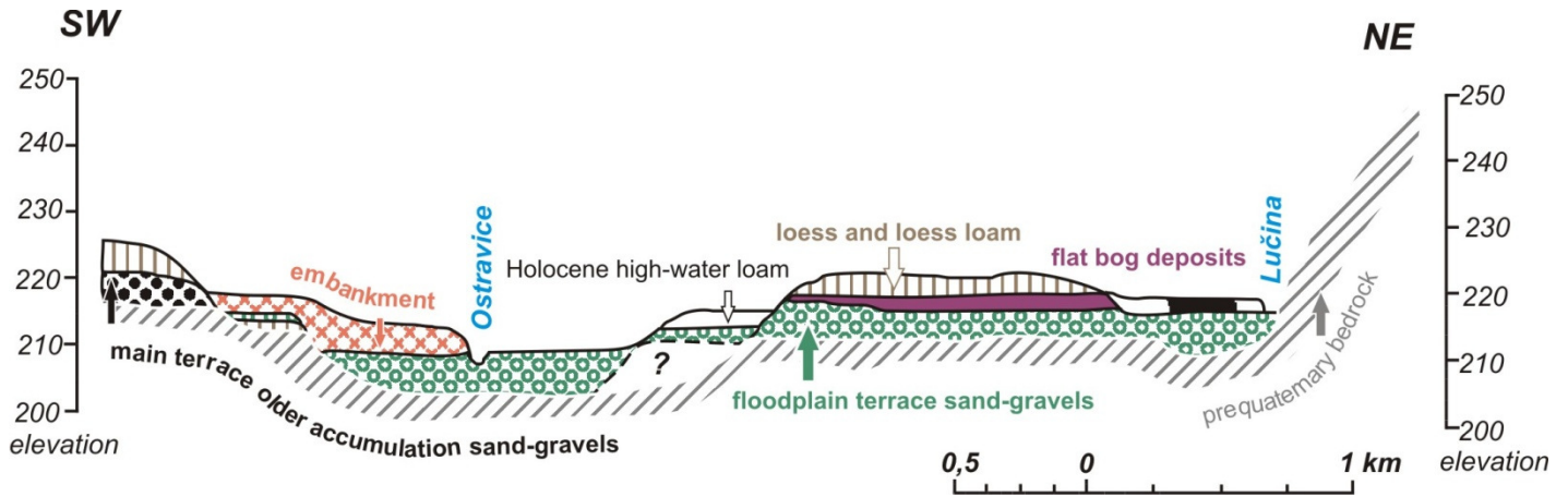
Figure 3. Schematical quaternary geological cross-section of part interest area in accordance with Macoun (1965).
