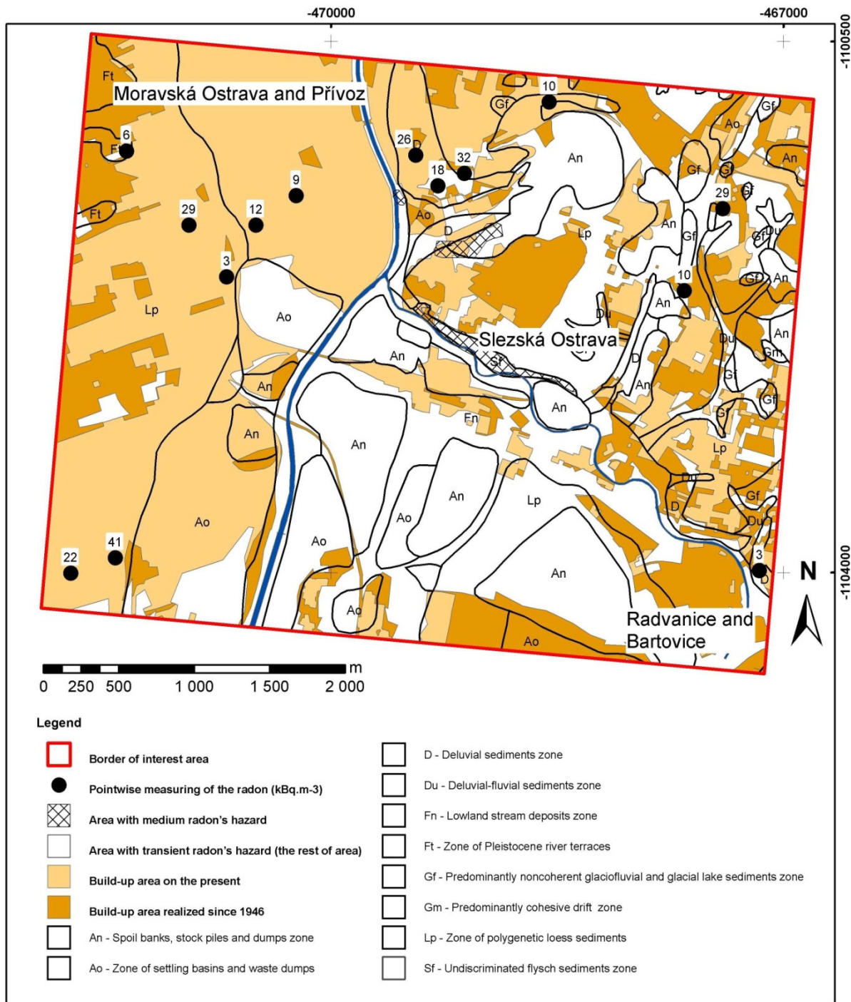
Figure 7. Map of radon hazard in the interest area with marked areal categories and point wise measuring of radon and marked engineering-geological zones of current built-up area and changes in the built-up area since 1946 to date - Radon data - (Czech Geological Survey, 2008).
