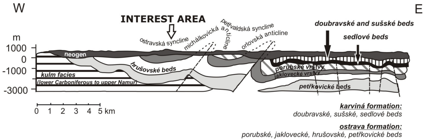
Figure 4. Schematical geological cross-section of interest area in accordance with Dopita (1997).
