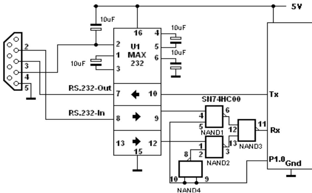
Figure 3. GSM pin connection to microcontroller.
