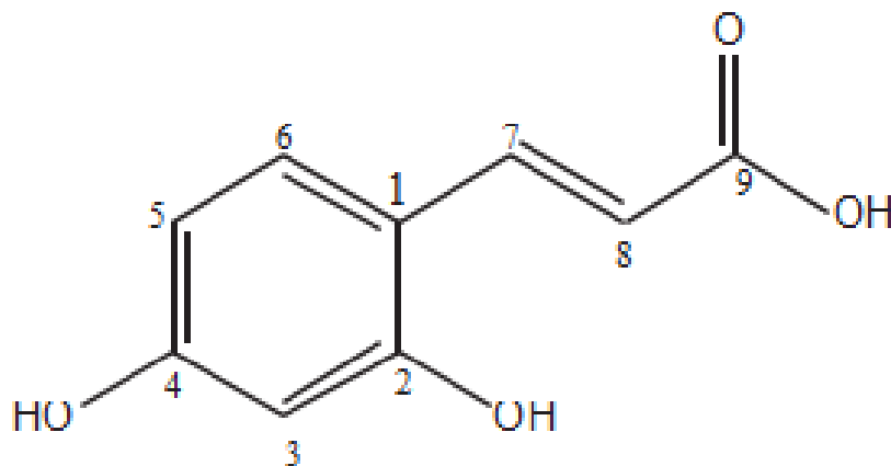
Figure 1. 2,4-dihydroxycinnamic acid.
